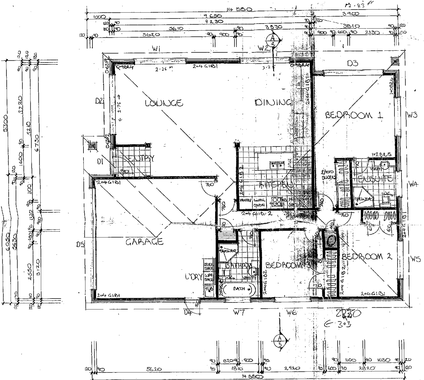
FLOOR PLAN 1:50 1570.5m 2
